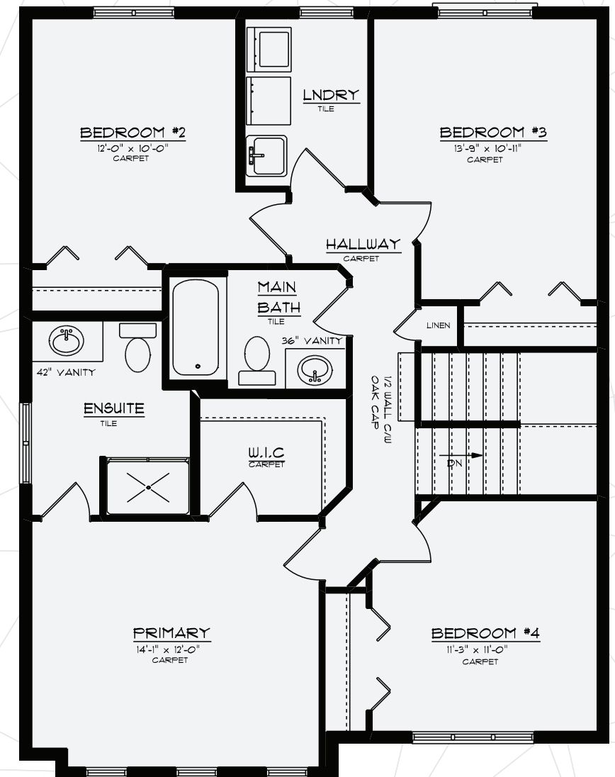
Upper Floor 1,064 Sq. Ft.
